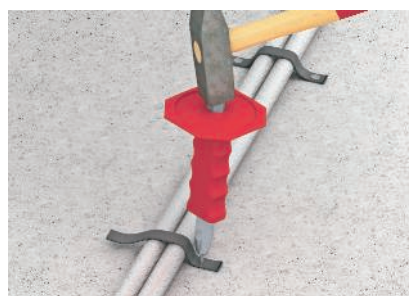
Pipe fixation by using fixpin with removable head and fabric strip
